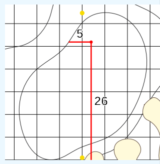
Hole 17 Depth 32
